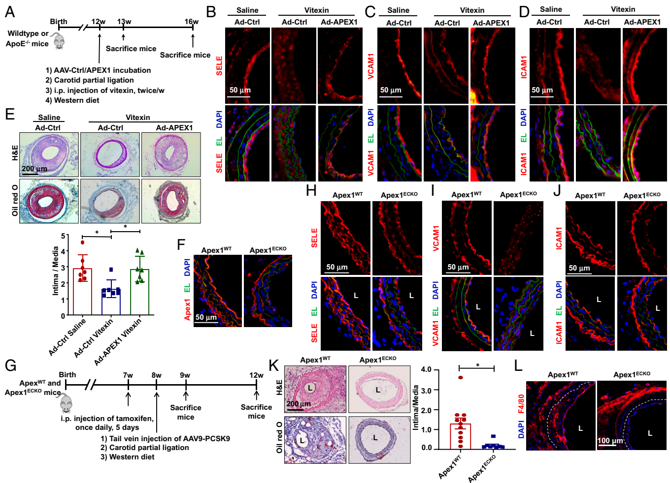
Fig. 7. Endothelial Apex1 contributes to the disturbed flow-accelerated atherogenesis. (A) Schematic diagram of experimental design. (B–D) Representative immunofluorescence staining of SELE (B), VCAM1 (C), and ICAM1 (D) in cross-sections of common carotid arteries from mice received vitexin or saline administration and were subjected to local intraluminal incubation with adenovirus-expressing APEX1 (Ad-APEX1) or control virus (Ad-CL) followed by partial ligation. Arterial specimens were harvested at 1-wk after the ligation ( n = 7 ). DAPI: to stain the nucleus; EL: elastic lamina. (E) Representative H&E and Oil red O staining and quantification of atherosclerosis in common carotid arteries from mice with treatments as described in A to D. Arterial specimens were harvested at 4 wk after ligation ( n = 7 ). Data are presented as mean \pm SEM, *P < 0.05 by the Kruskal–Wallis test followed by Dunn’s test. (F) Representative immunofluorescent staining of APEX1 in carotid arteries from Apex1 WT or Apex1 ECKO mice receiving tamoxifen to verify Apex1-depletion. (G) Schematic diagram of experimental design. (H–J) Representative immunofluorescence staining of SELE (H), VCAM1 (I), and ICAM1 (J) in cross-sections of the left common carotid arteries from the Apex1 WT or Apex1 ECKO mice. Arterial specimens were harvested at 1-wk after ligation. (K) Representative H&E and Oil red O staining and quantification of neointima in the left common carotid arteries from the Apex1 WT or Apex1 ECKO mice. (L) Representative immunofluorescent staining of F4/80 indicative of monocyte infiltration in the left common carotid arteries from the Apex1 WT or Apex1 ECKO mice. Arterial specimens in K and L were harvested at 4-wk after ligation ( n = 7–11 ). *P < 0.05 by the Mann–Whitney test. L: lumen.
